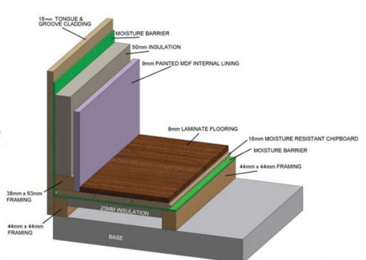
Oxford & Winchester Apex, Henley & Canterbury Pent, Cheltenham & Dorchester Corner Pent wall & floor specification with 50mm insulation
