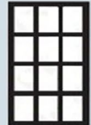
12 PANE WIDTH - 745MM HEIGHT - 1375MM WGF12
